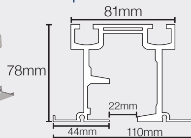
Slide & Stack 3m Top Track
