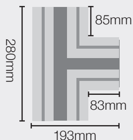
Slide & Stack T Junctions
