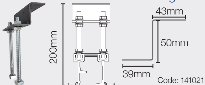
Track Bracket M12x 149mm Long Studs
