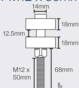
Double Roller M12 x 50mm Thread
