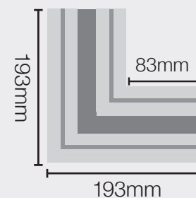
Slide & Stack L Junctions
