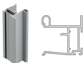
(G) 2.7 Metre side handle housing profile
