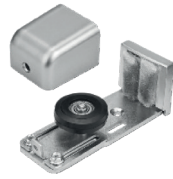
Floor guide
