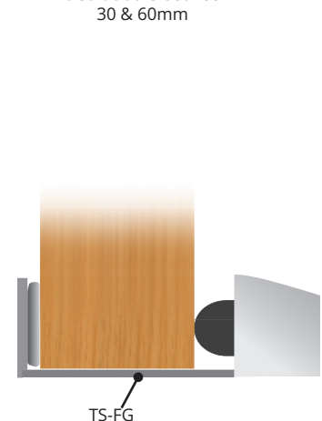
Floor guide To suit doors between 30 & 60mm
