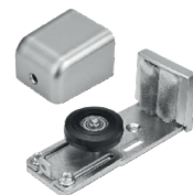
Code: TS-FG To suit doors between 30 & 60mm
