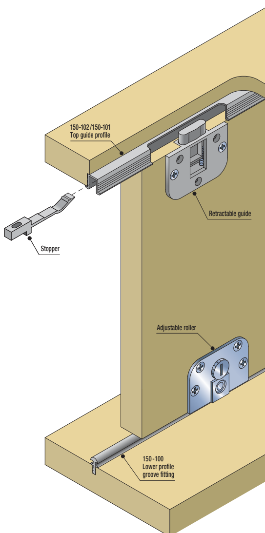
2x Adjustable Rollers
