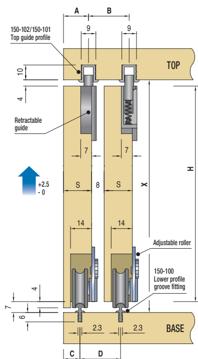
2x Retractable Guides
