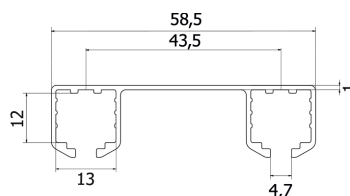
Surface Fixed
