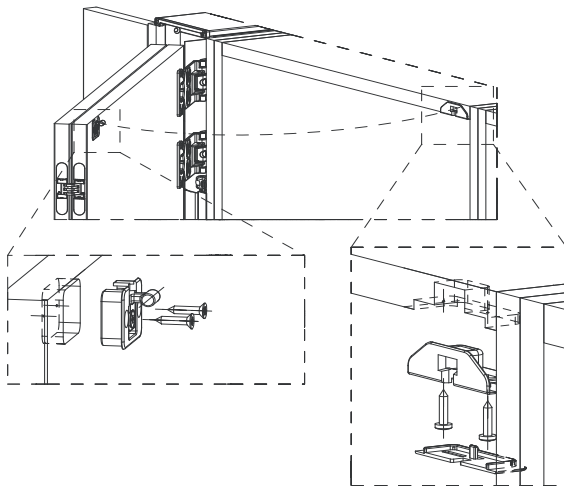
Adjustable Door Support Pin (Optional) 750-510
