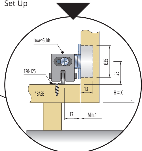
Alternative Bottom Guide Set Up
