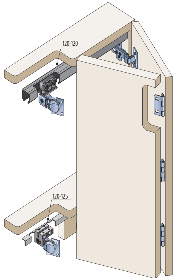
Alternative Bottom Guide Set Up
