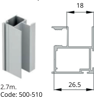
Side handle profile:
