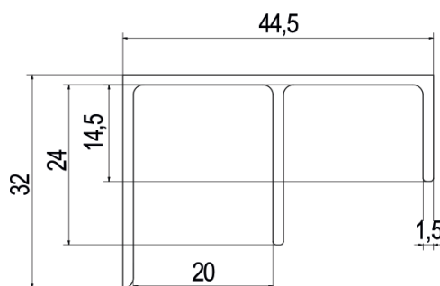
2x Lower Guide (B)
