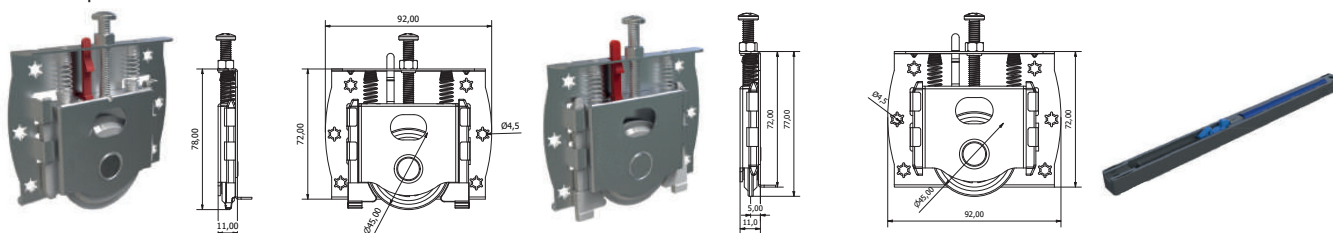
Top guides
