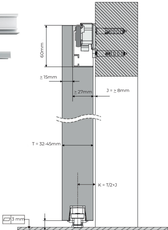
Lower runner
