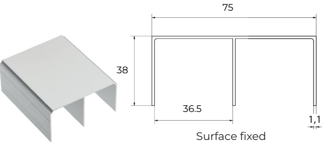
(A) 3000 mm top track Code: 500-101-3
