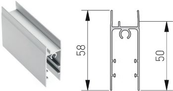
(H) 3000 mm bottom frame/roller housing Code: 500-320
