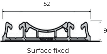
(B) 3000 mm bottom track Code: 500-109-3
