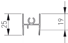
(F) 3000 mm Top frame/roller housing profile Code: 500-321
