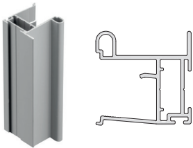
(G) 2700 mm side handle housing profile Code: 500-418
