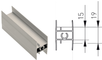
(J) 3000 mm bolt-on middle panel connector Code: 500-319
