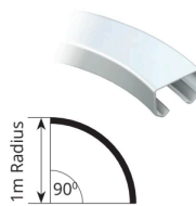
1m Radius curved top track Code: 20-285
