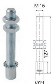
Bottom guide roller with thread Code: 300-791
