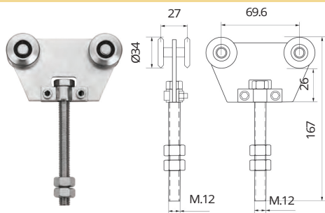
Double axle hanger, 150kg capacity Code: 300-469
