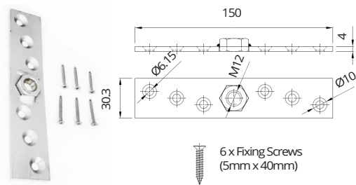
Grade suspension plate set for wooden doors, pair Code: 450-46011
