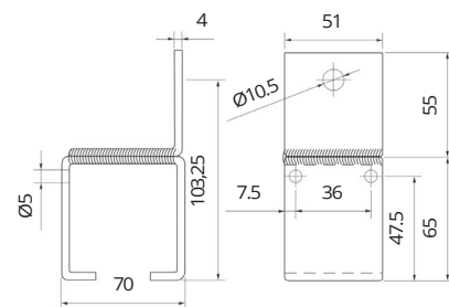
Face fix bracket Code: 450-47950
