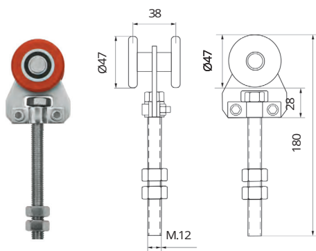
Single axle 120kg capacity Code: 450-483
