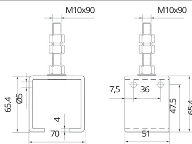
Adjustable bracket Code: 450-47960
