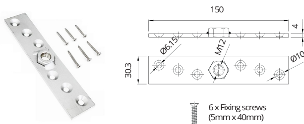
Grade suspension plate set for wooden doors, pair Code: 450-46011
