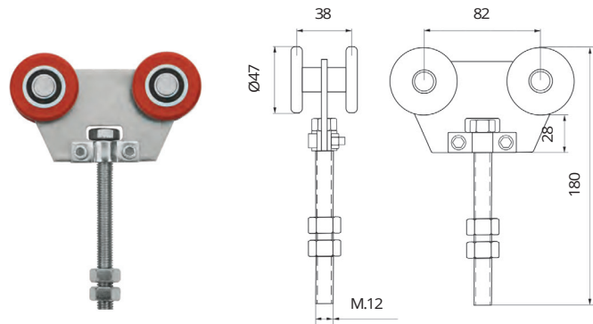
Double axle 225kg capacity Code: 450-484
