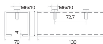
Top track connector Code: 450-47911
