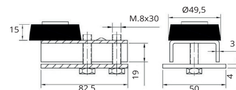
Track mounted door stop Code: 450-47501
