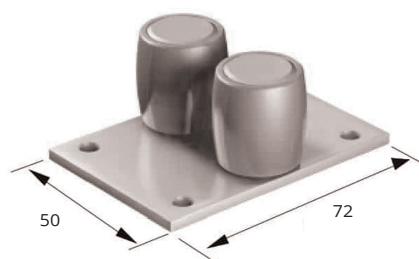
25mm Diameter double bottom guide roller, on flat plate Code: 250-77
