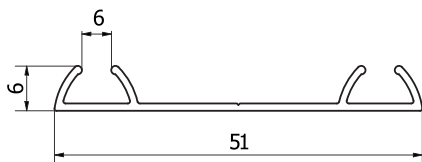
Recess Fix
