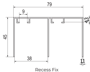
Recess Fix
