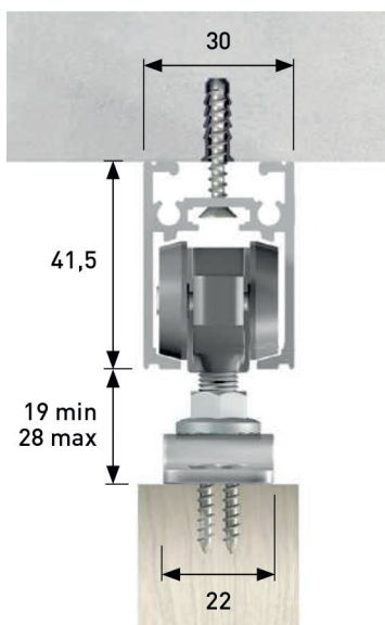
Soffit fixing
