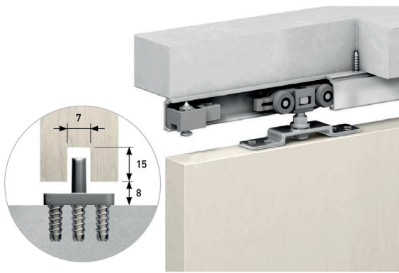
Soffit fixing
