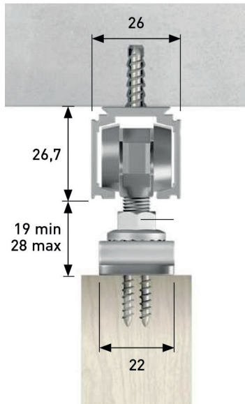
Soffit fixing
