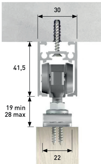
Soffit fixing
