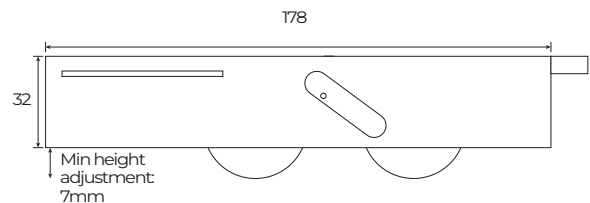
Nylon twin roller unit - 90kg capacity (Maximum Adjustment: 193mm) Code: 100-202
