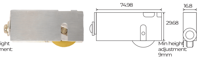
Single brass roller unit - 35kg capacity (Maximum Adjustment: 93mm) Code: 100-201
